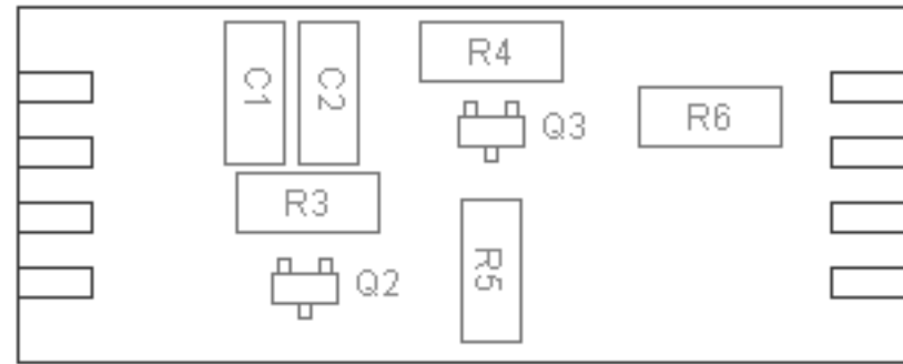
Bottom side (viewed from top)
